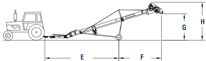
TRANSPORT POSITION
